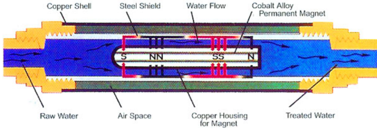
SUPERIOR WATER CONDITIONER CROSS SECTIONAL VIEW
